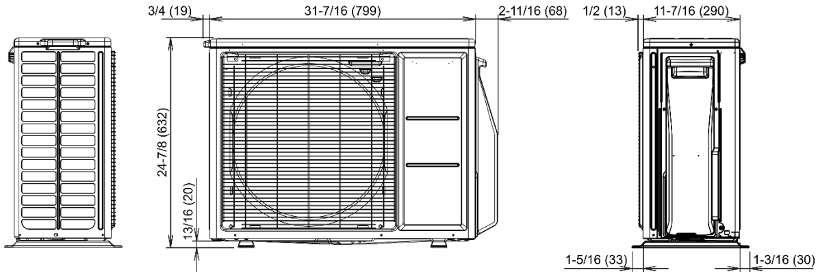
Side view
