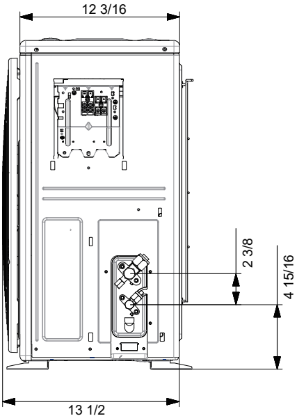
RIGHT (pictured without valve/wire cover)
