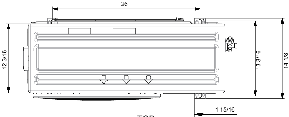
TOP (pictured without valve/wire cover on right side)
