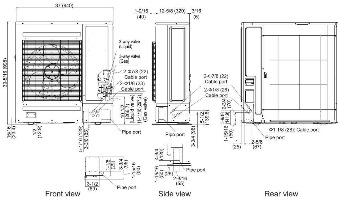
Front view
