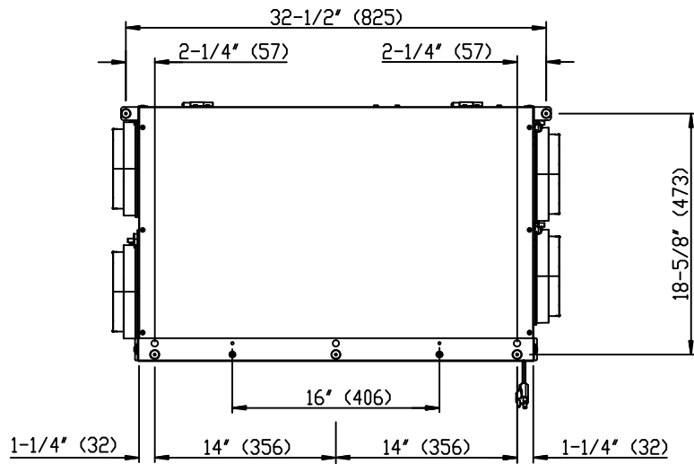
Hanging Hole Pattern (Bracket) Top View
