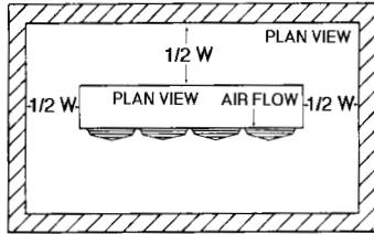
One evaporator
