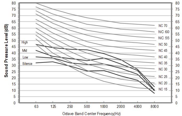
4) CNH36TDB (AC036BNTDCH/AA)
