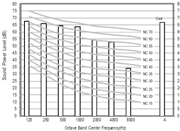
3) CXC30SCB (AC030BXSCCC/AA)
