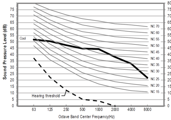
3) CXC30SCB (AC030BXSCCC/AA)
