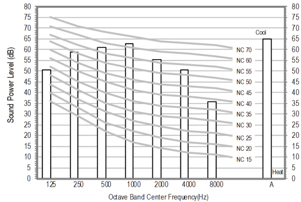
4) CNH36TDB (AC036BNTDCH/AA)
